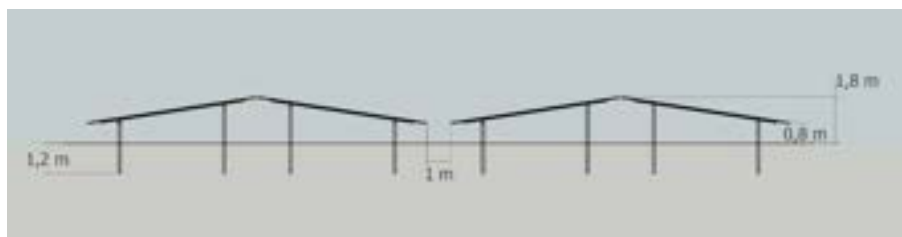
Figur 5. Illustration af Fixed-tilt E/W
